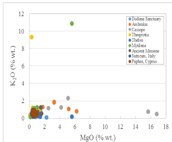
Fig. 3: The majority of samples belong to the natron area (K 2 O, MgO <1% wt.) while there are few exceptions.
