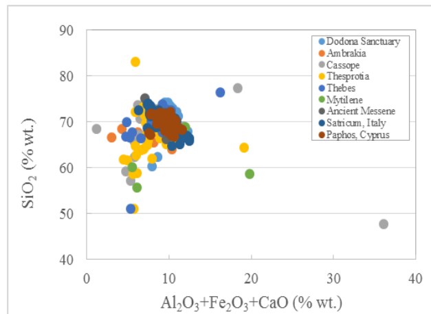
Fig. 2: Correlation between SiO 2 and the sum of Al 2 O 3 +Fe 2 O 3 +CaO might indicate possible different sand raw materials.
