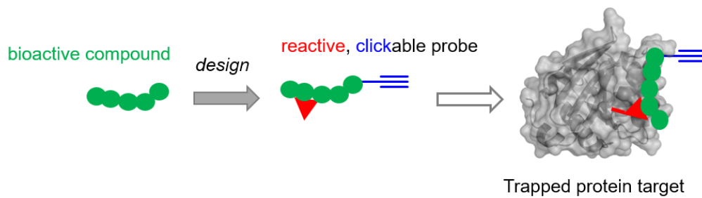
Figure 1: The chemical proteomics approach used in this research. A probe is designed based on a bioactive compound (in this case, DYN). The probe consists of a photoreactive group (red) and a clickable tag (blue). Upon binding to its protein target and UV irradiation, the photoprobe crosslinks to the protein target. The tag can later be used to isolate the protein for identification.
