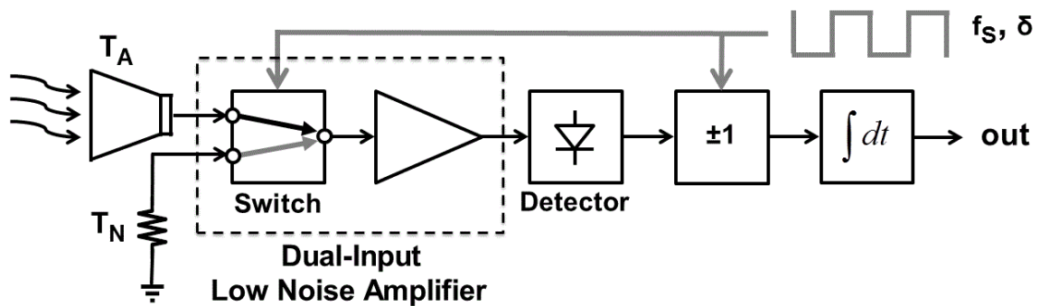
Fig. 1.2. Block diagram of the SoC radiometer
