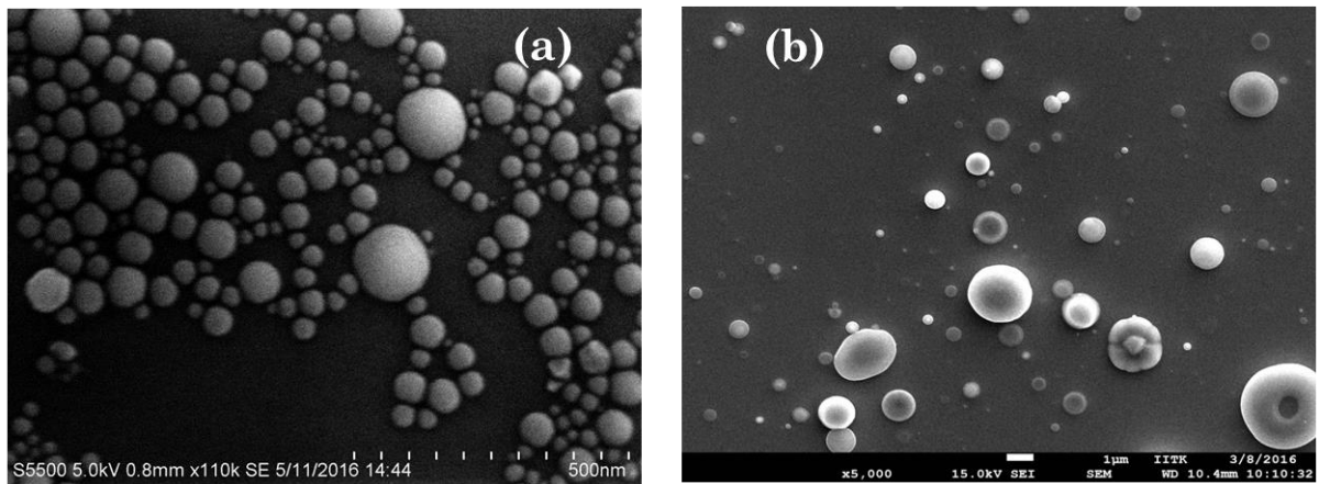
Figure 3. (a) Deposited metallic (Al) nanoparticles and (b) deposited nanocomposites (Cu-TiO 2 ) on silicon substrate from stagnation layer.
