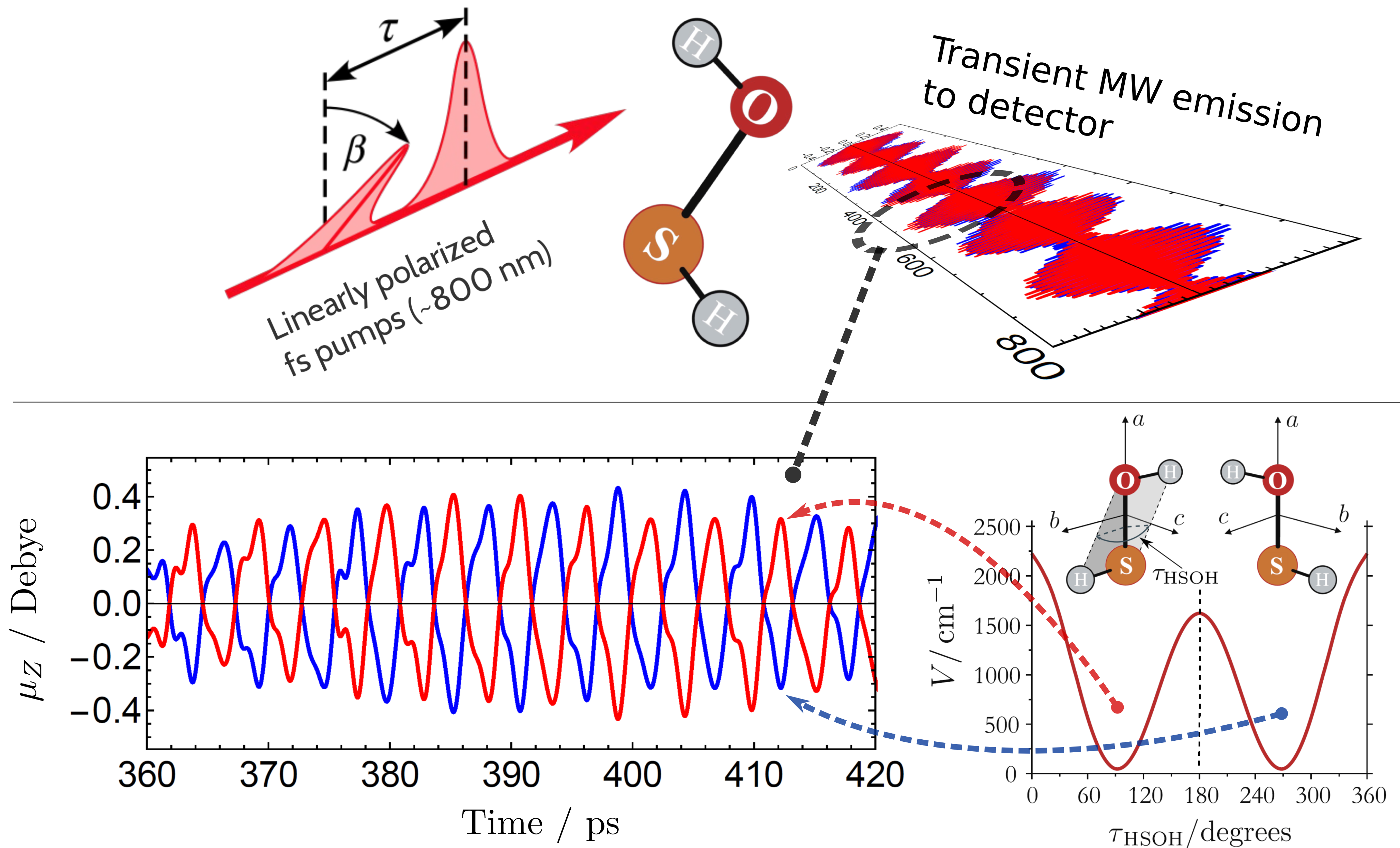
Fig. 4: Two-pulse enantiomer differentiation scheme and calculated time evolution of the electric dipole moment for two enantiomeric forms of HSOH
