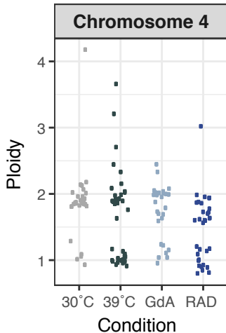
Figure 1: Hsp90 disturbances cause LoH and aneuploidy. LoH events detected on chromosome 4 differ between environmental stressors (left). Hsp90 inhibition causes haploidy (right).
