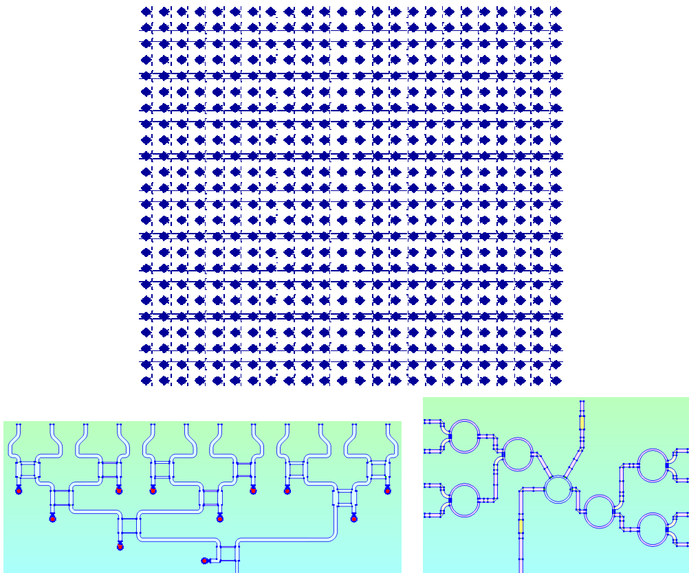
Antenna e.m. model
