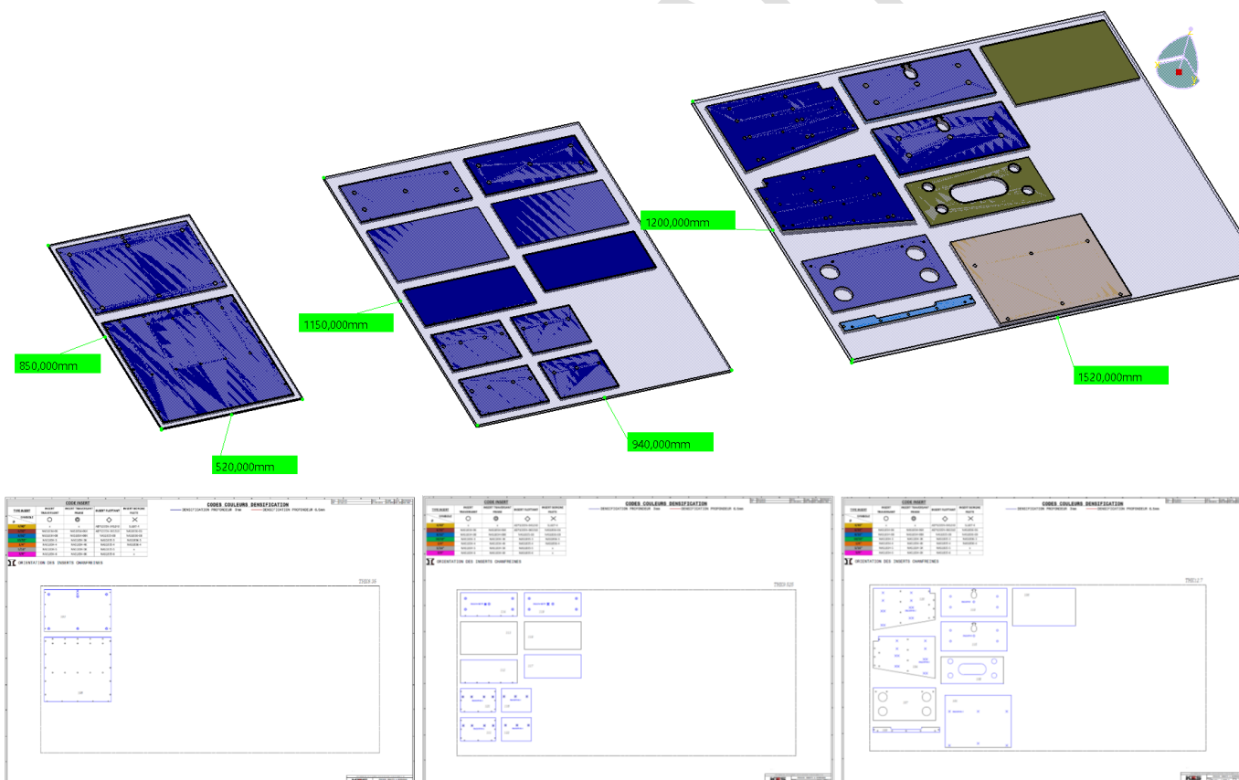
Figure 8 : Panels imbrication and manufacturing process insert instruction
