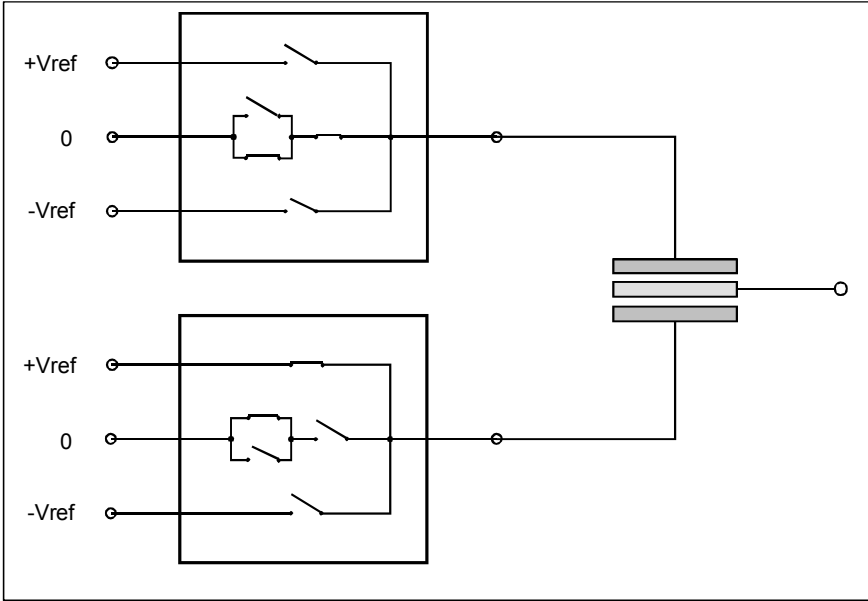
Fig. 3: Block structure of the switch unit
