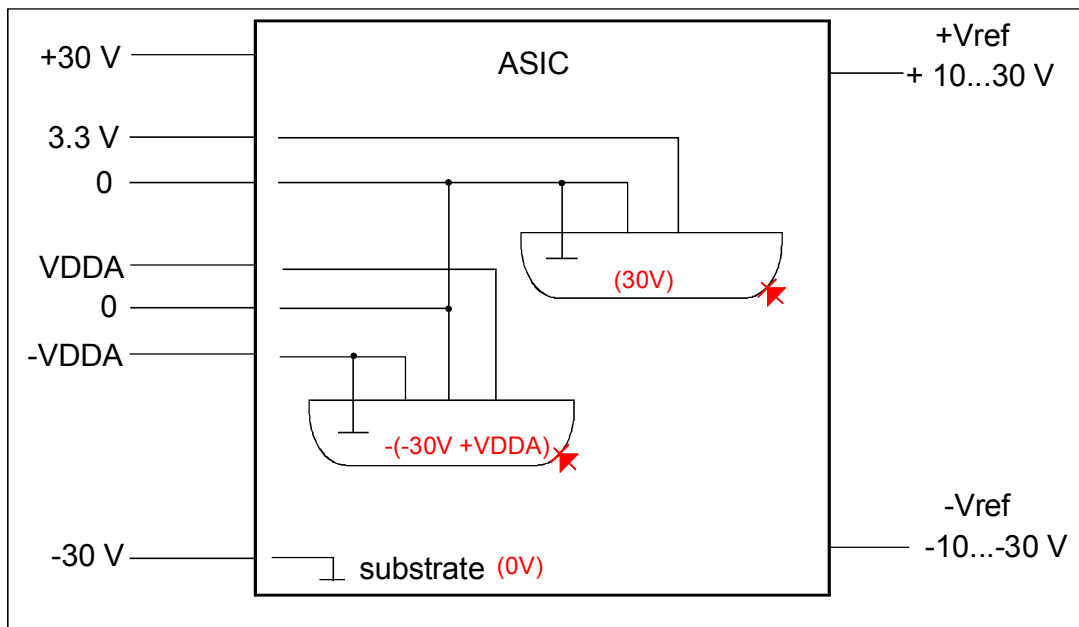
Fig. 2: Power supply
