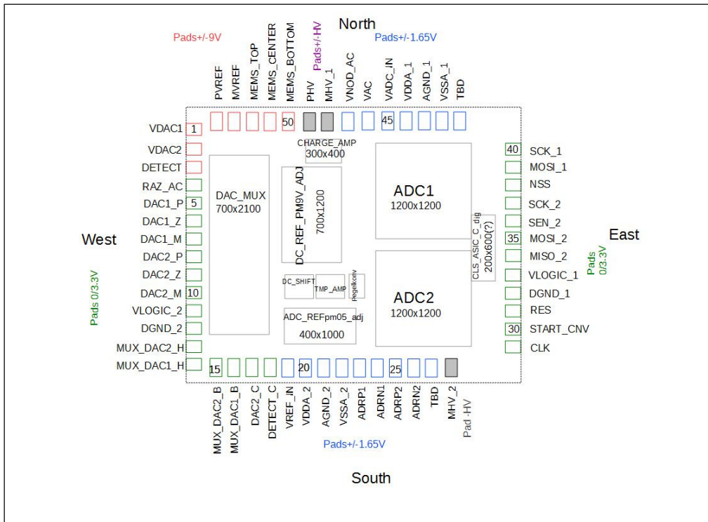
Fig. 6: ASIC C - Floorplanning
