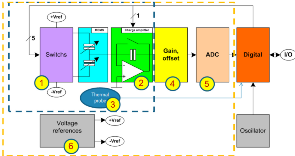
Fig. 1: Block structure of the MEMS-based accelerometer for detection of wing deformations
