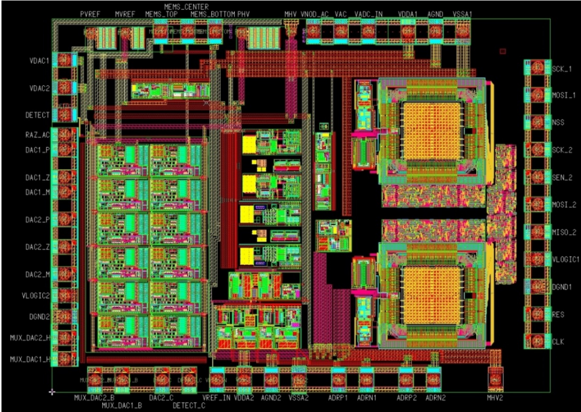
Fig. 7: ASIC C – Final layout
