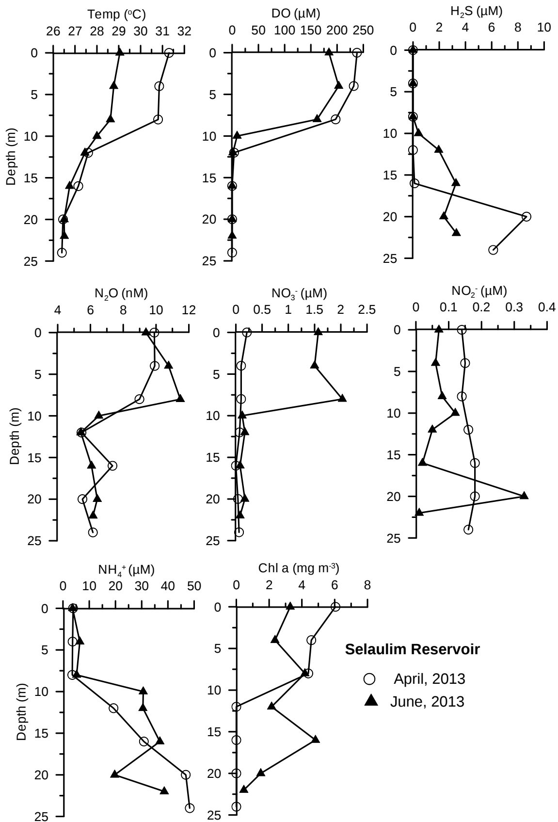
Figure1- Vertical profiles of temperature, DO, H 2 S, N 2 O, NO 3 - , NO 2 - , NH 4 + and Chl a in Selaulim Reservoir during April and June, 2013.
