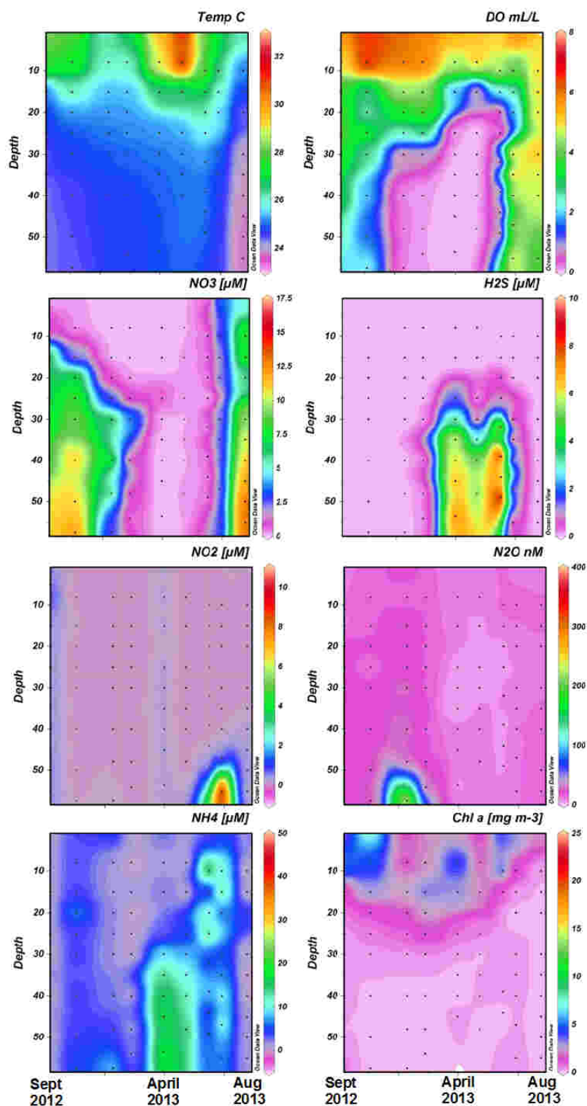
Figure 2- Time series data of temperature, DO, H 2 S, NO 3 - , NO 2 - , NH 4 + , N 2 O, and Chl a collected from Tillari reservoir during September 2012 to August 2013.
